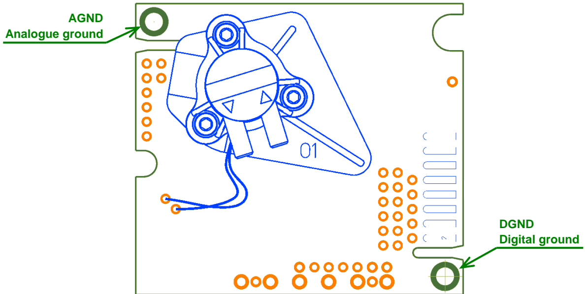
Figure 4. CO 2 Engine ® ICB-F ground / shield attachment
